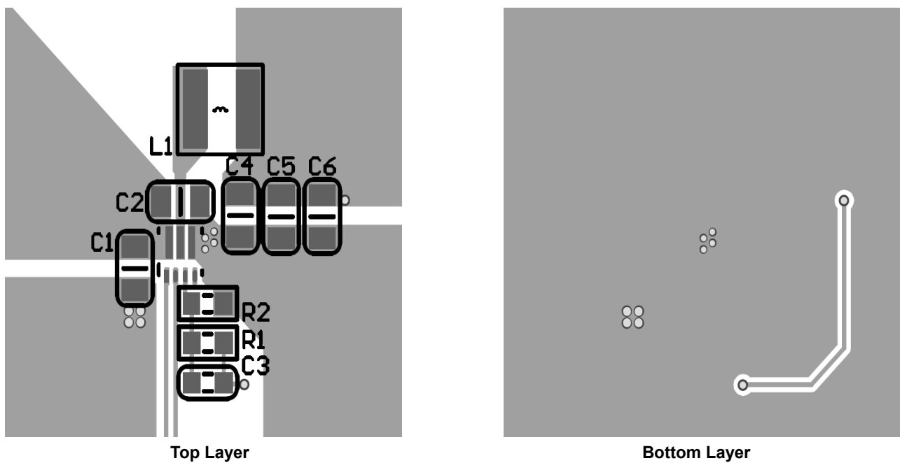
Figure 4. PCB Layout
