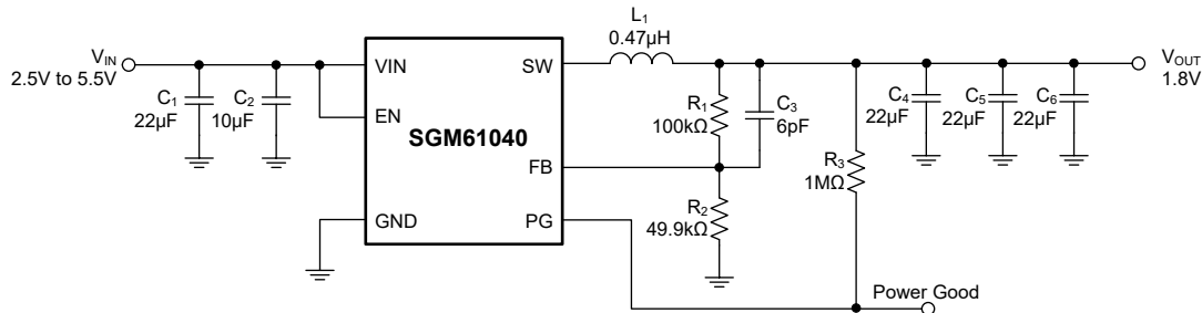
Figure 3. SGM61040 Circuit for 1.8V Output
