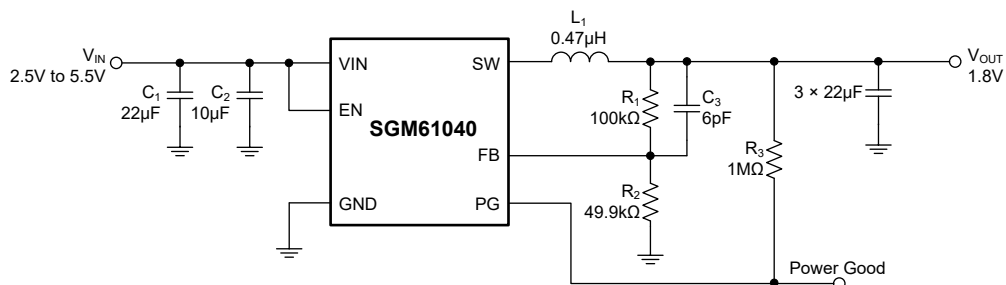
Figure 1. SGM61040 Typical Application Circuit
