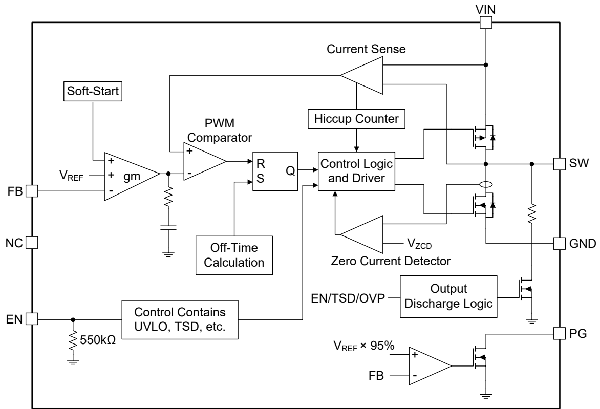
Figure 2. SGM61040 Block Diagram
