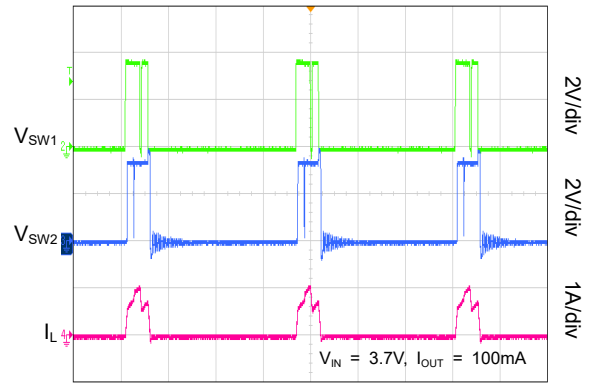
Time (2µs/div)
