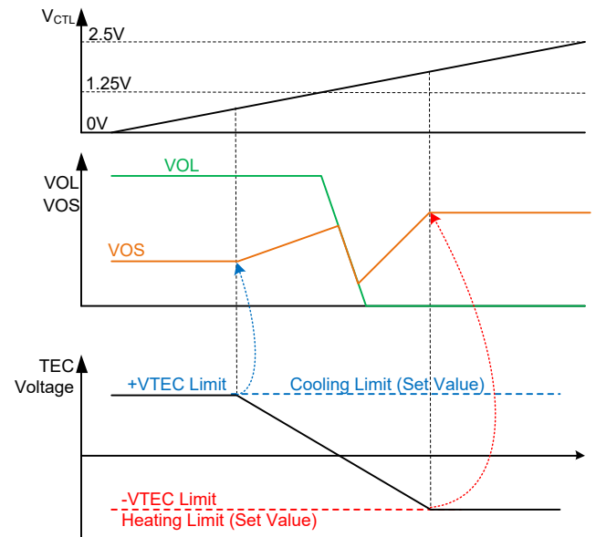
Figure 5. Primary TEC Voltage Limit Protection
