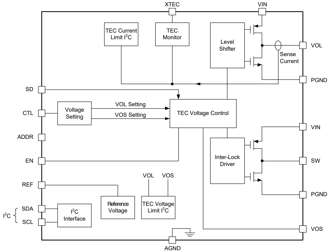
Figure 2. Block Diagram
