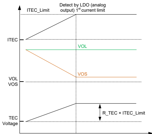
Figure 7. Primary Current Limit Protection (1 st Limit)
