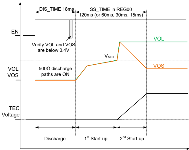
Figure 4. Three-Step Soft-Start of the Power Stage
