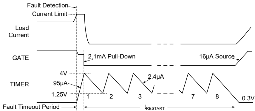
Figure 7. Restart Sequence
