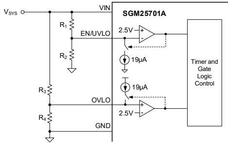
Figure 10. Programming the Four Thresholds
