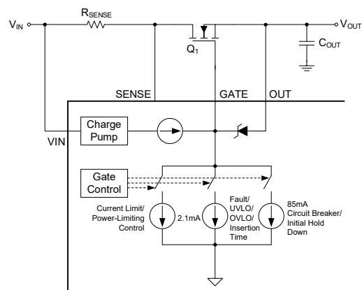
Figure 5. Gate Control
