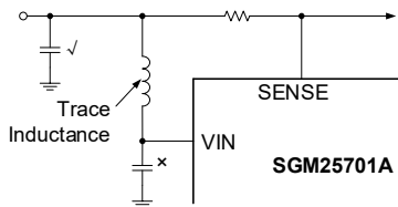
Figure 11. Layout Trace Inductance
