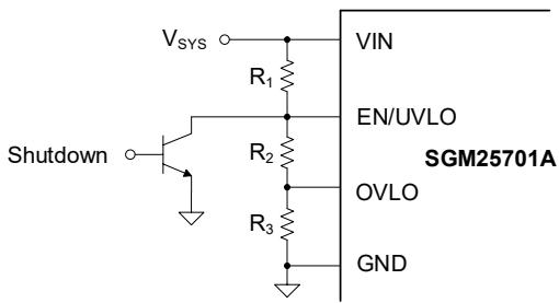
Figure 6. Shutdown Control
