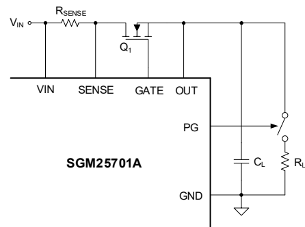
Figure 9. No Load Current during Turn-On
