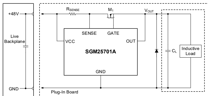
Figure 12. Output Diode Required for Inductive Loads
