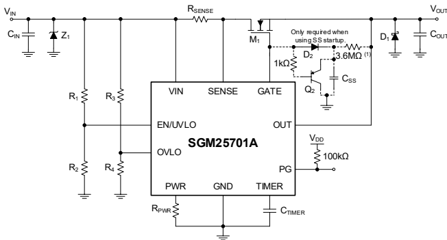
Figure 8. Typical Application Schematic (36V/11A)
