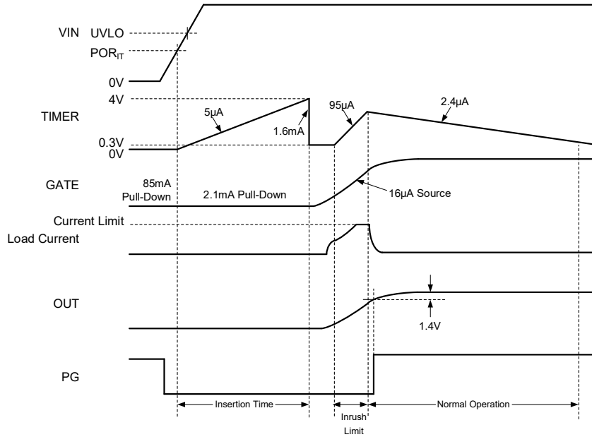
Figure 4. Power-Up Sequence (Power-Limiting Only)
