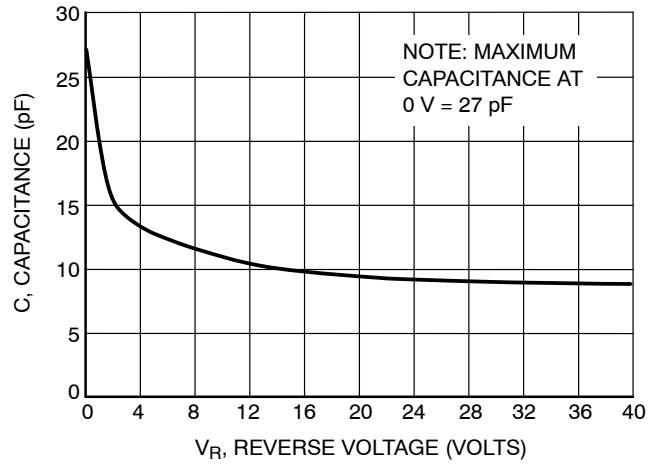
Figure 6. Maximum Capacitance
