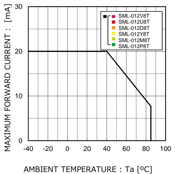
Fig.4 Derating
