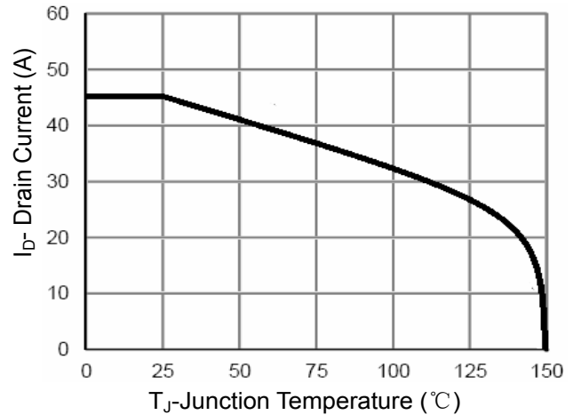
Figure 10 Current De-rating
