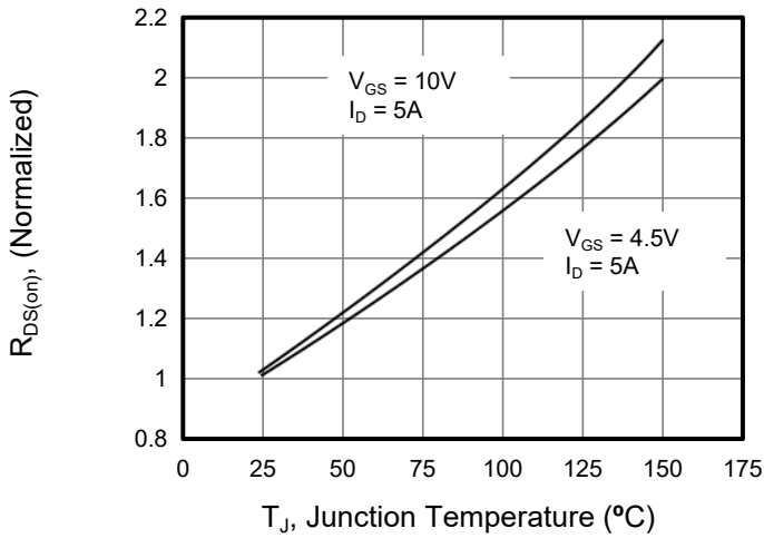
Figure 7. Drain-Source On-Resistance
