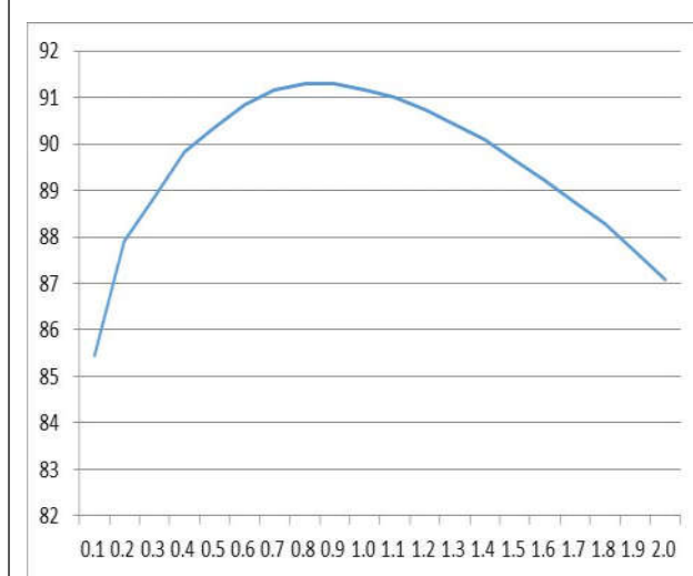
The efficiency for VOUT=3.3V
