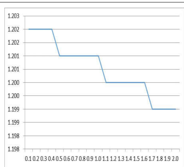
The Load Regulation For VOUT=1.2V
