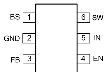
TD8112 (SOT23-6)
