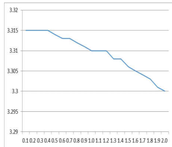
The Load Regulation For VOUT=3.3V
