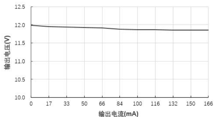
输出电压 VS 输出电流 IB1212S-2W@ (Vin=12V)
