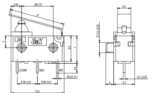
L14 LEAF LEVER WITH LEVER LENGTH 14 MM
