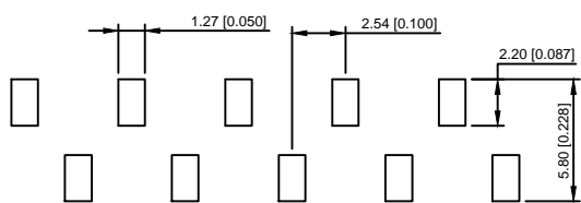
PCB LAYOUT R1 TYPE
