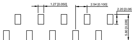
PCB LAYOUT R1 TYPE
