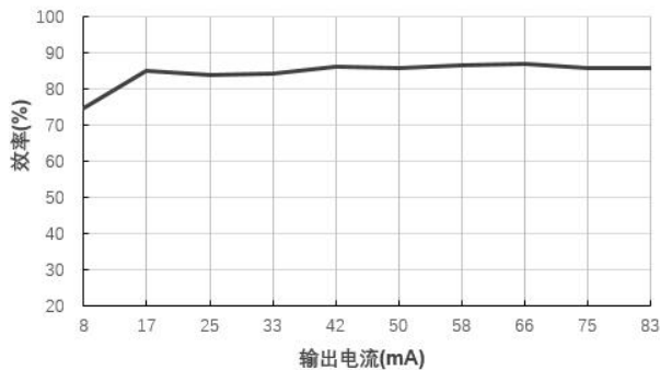
效率Vs输出电流(Vin=5V)@B0512LS-1WR2
