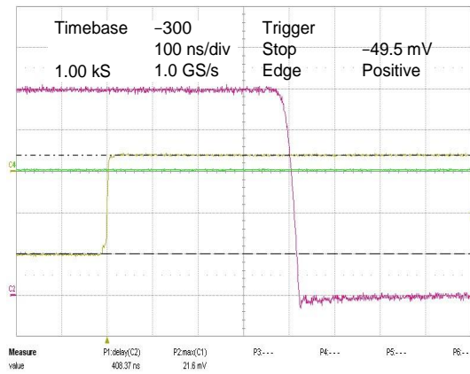
Figure 17. 20 mV Overdrive
