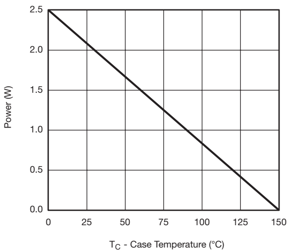
T_C - Case Temperature (°C) Power Derating, Junction-to-Foot
