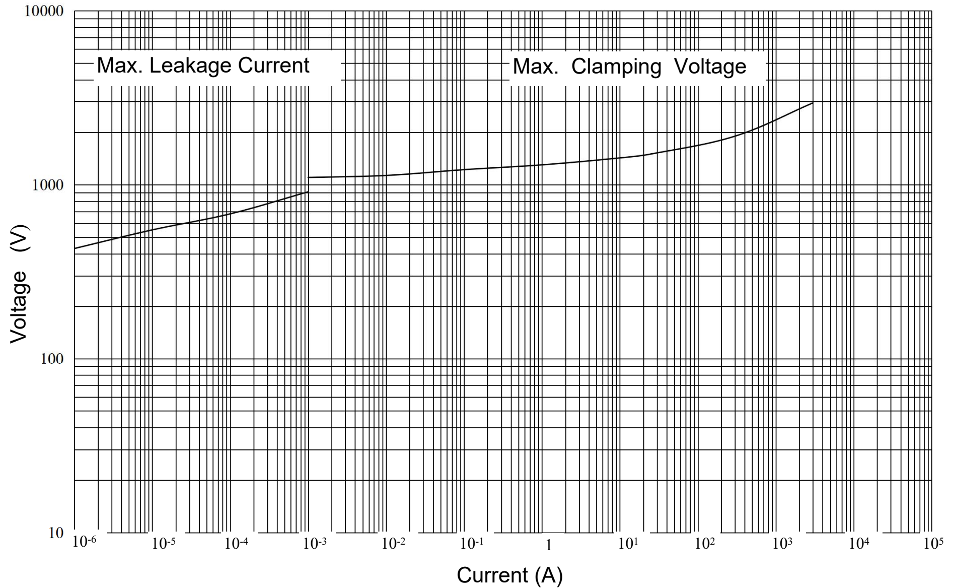
TVR10911KS221Y
