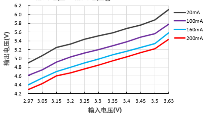
输出电压Vs输入电压@B0305LS-1WR2
