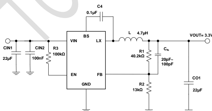
STI3452I Typical Application Circuits
