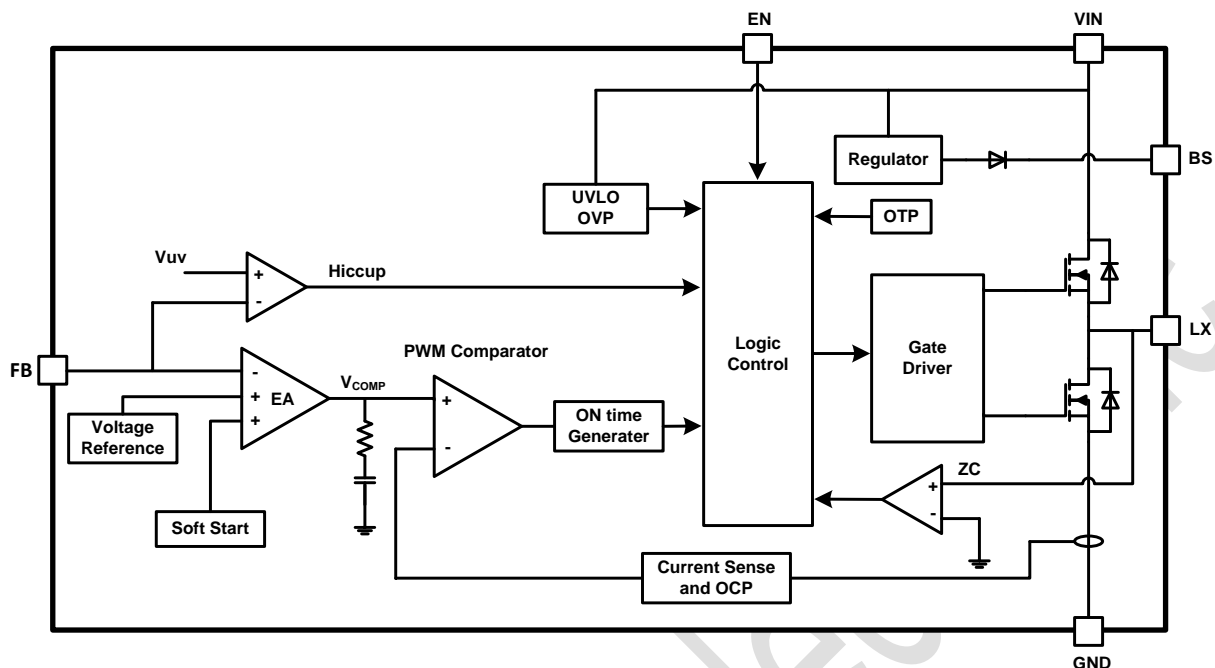
Figure 1. STI3452I Block Diagram
