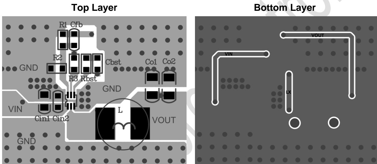
Figure 3. Sample of PCB Layout (STI3452I)
