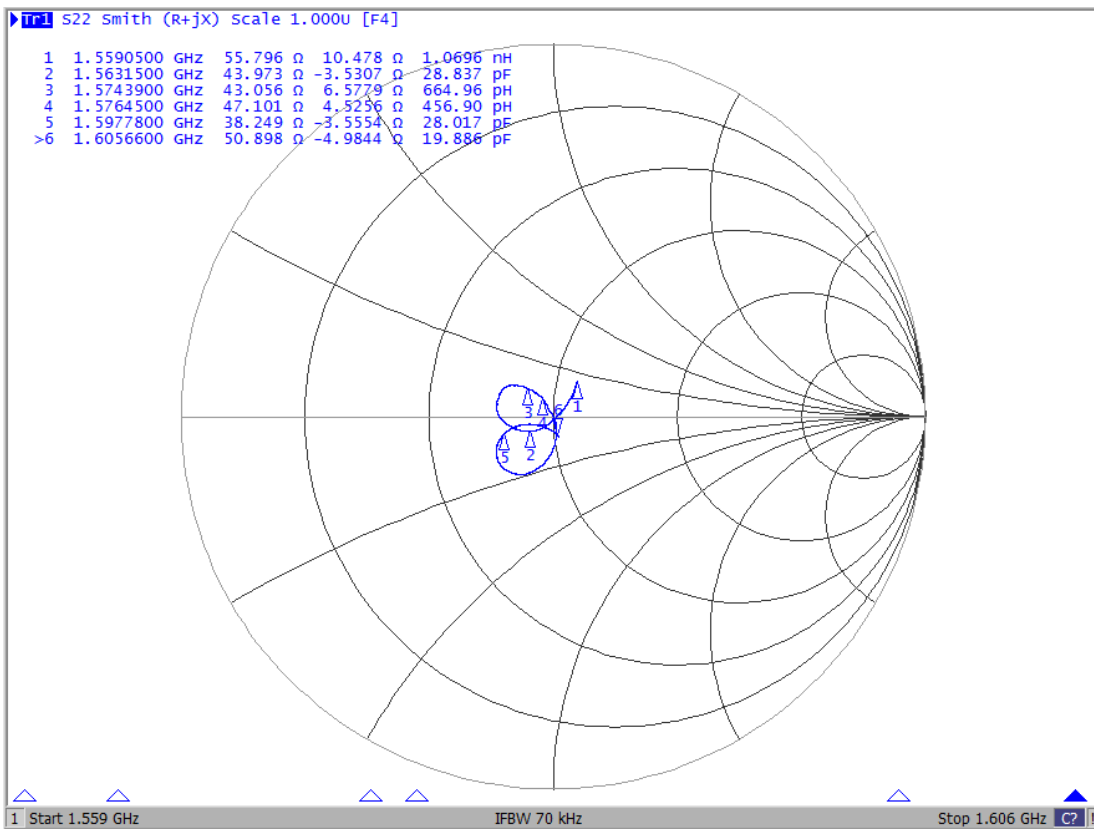
Figure 6: Reflection coefficient for S22
