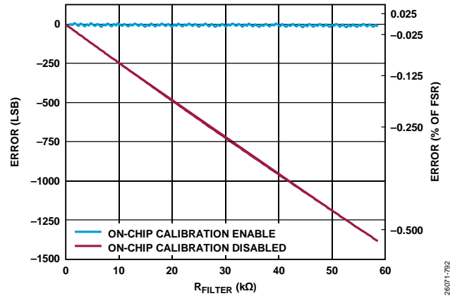
Figure 93. System Gain Calibration, With and Without Calibration, \pm 10 V Single-Ended Range
