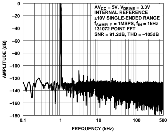
Figure 10. FFT, ±10 V Single-Ended Range, Low Bandwidth Mode
