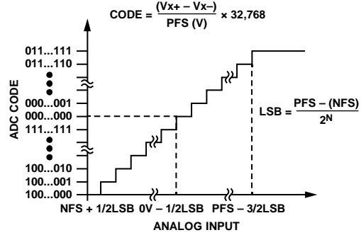
Figure 81. AD7606C-16 Ideal Transfer Characteristics, Bipolar Analog Input Ranges (Twos Complement Output Coding)
