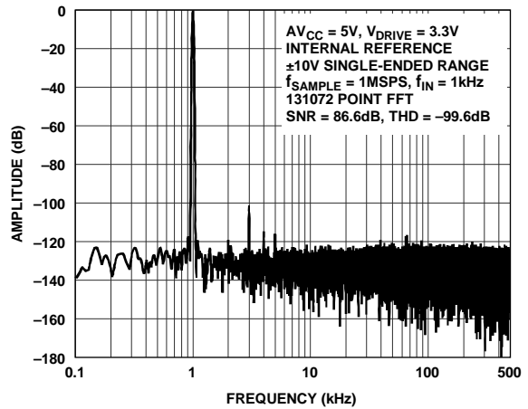
Figure 13. FFT, ±10 V Single-Ended Range, High Bandwidth Mode
