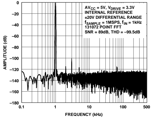
Figure 12. FFT, ±20 V Differential Range, High Bandwidth Mode
