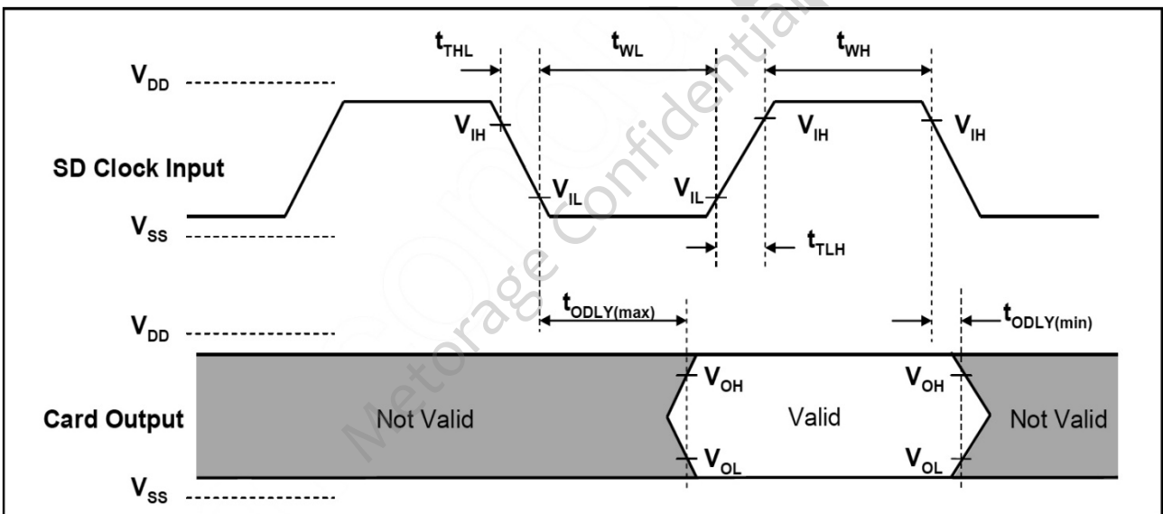
Figure 6-5 Card Output Timing (Default Speed Card)
