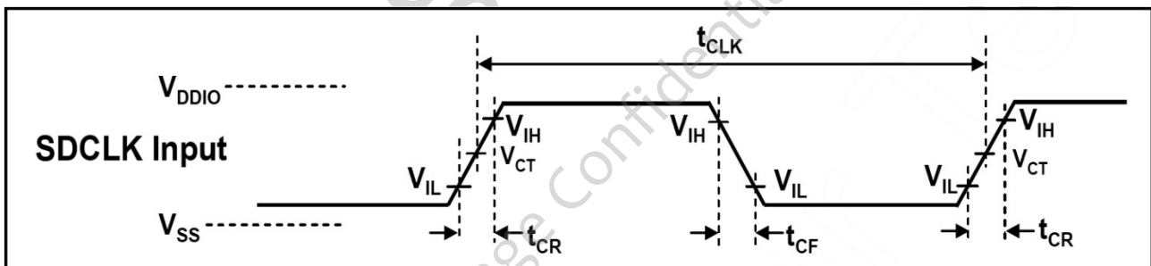
Figure 6-8 Clock Signal Timing
