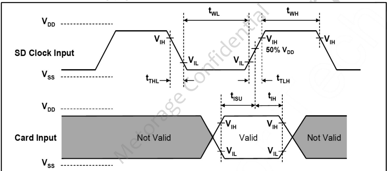
Figure 6-6 Card Input Timing (High Speed Card)
