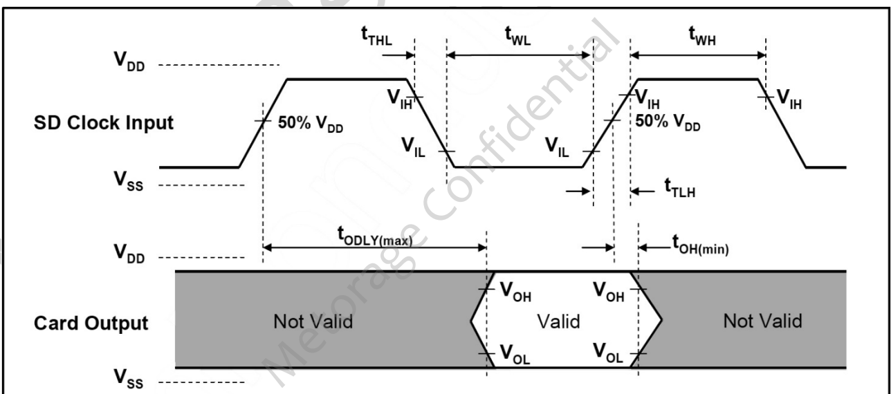
Figure 6-7 Card Output Timing (High Speed Mode)
