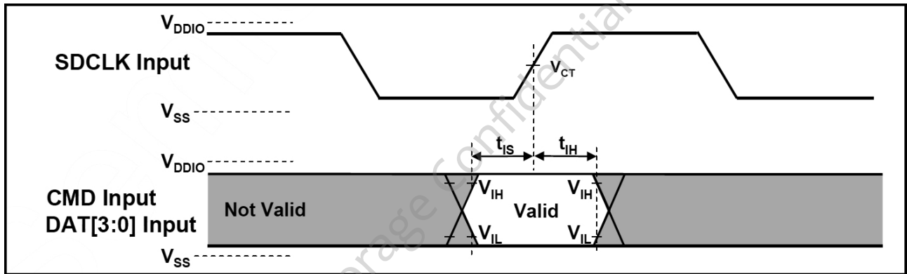
Figure 6-9 Card Input Timing
