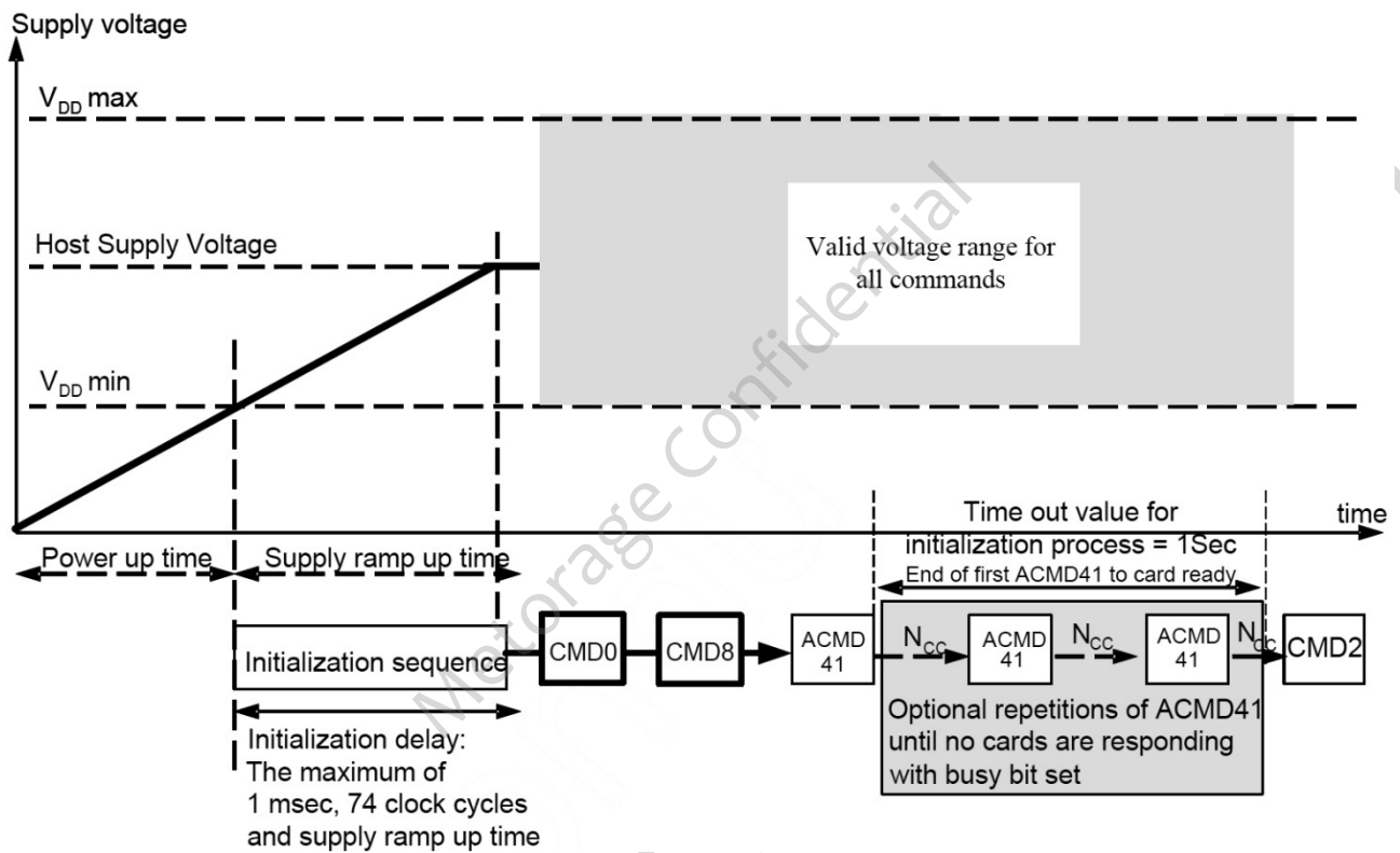
Figure 6-2 Power Up Diagram of Card
