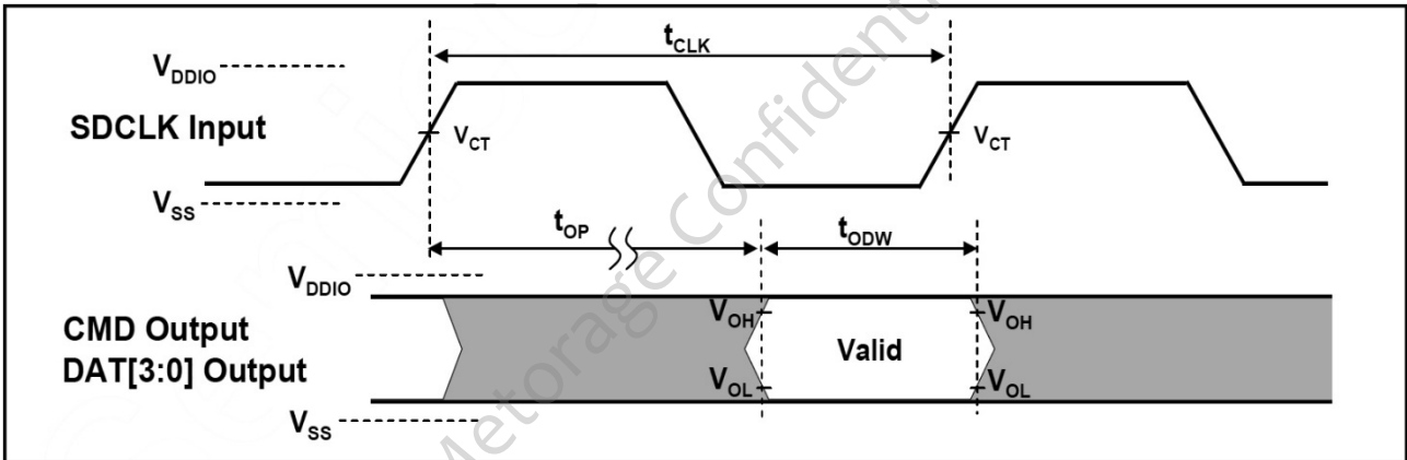
Figure 6-11 Output Timing of Variable Data Window
