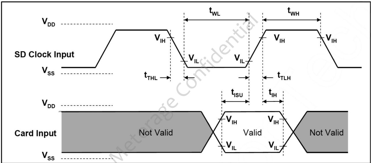
Figure 6-4 Card Input Timing (Default Speed Card)
