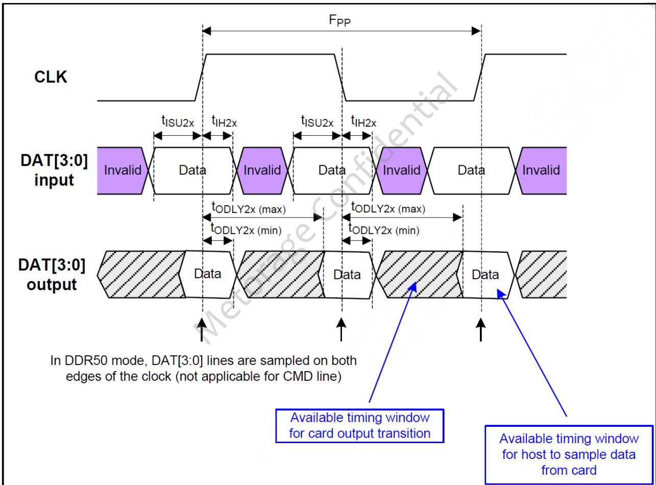
Figure 6-13 Timing Diagram DAT Inputs/Outputs Referenced to CLK in DDR50 Mode
