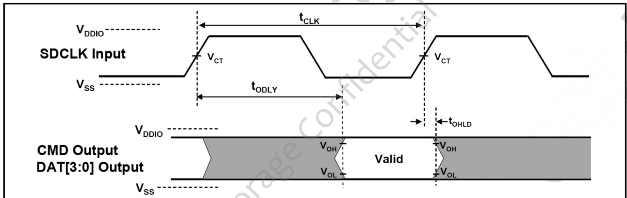
Figure 6-10 Output Timing of Fixed Data Window
