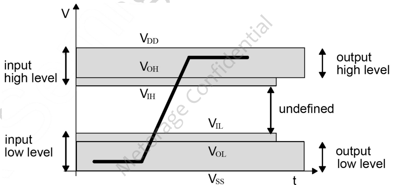
Figure 6-3 Bus Signal Level
