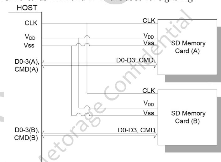
Figure 3-2 SD Memory Card System Bus Topology
