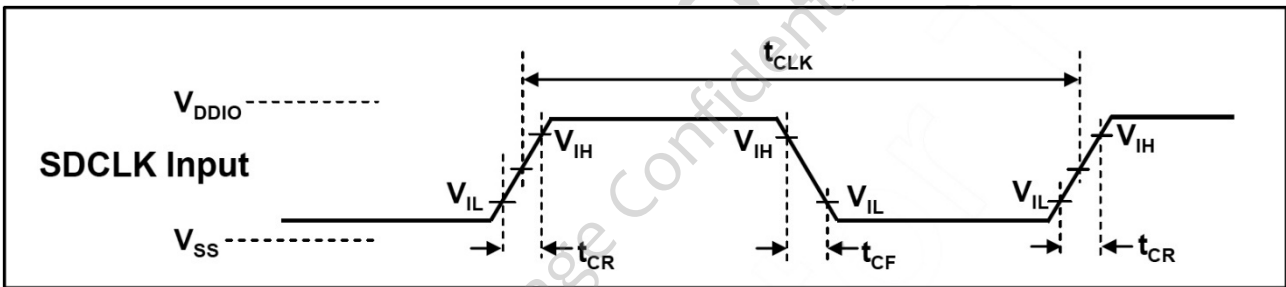
Figure 6-12 Clock Signal Timing
