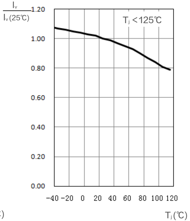
相对发光强度 / Relative Luminous Intensity I_v/I_v(25^\circ\text{C}) = f(T_j); I_f = 10\text{ mA}
