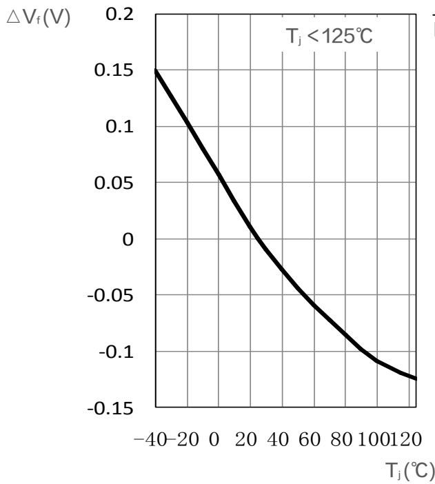
相对正向电压 / Relative Forward Voltage \Delta V_f = V_f - V_f(25^\circ\text{C}) = f(T_j); I_f = 10\text{ mA}
