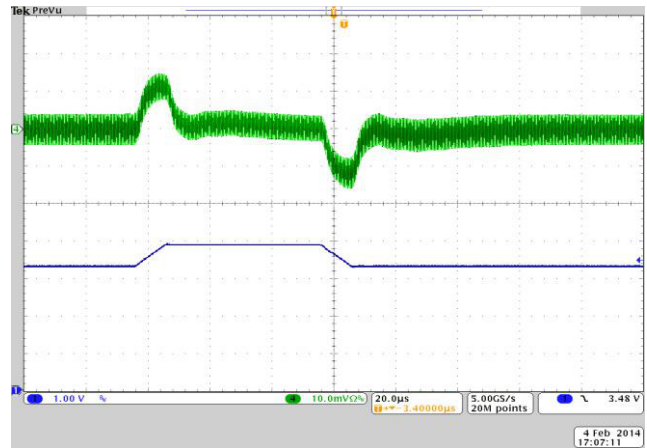
Figure 14. Line Transient, 200 mA Load, 10 μs Step
