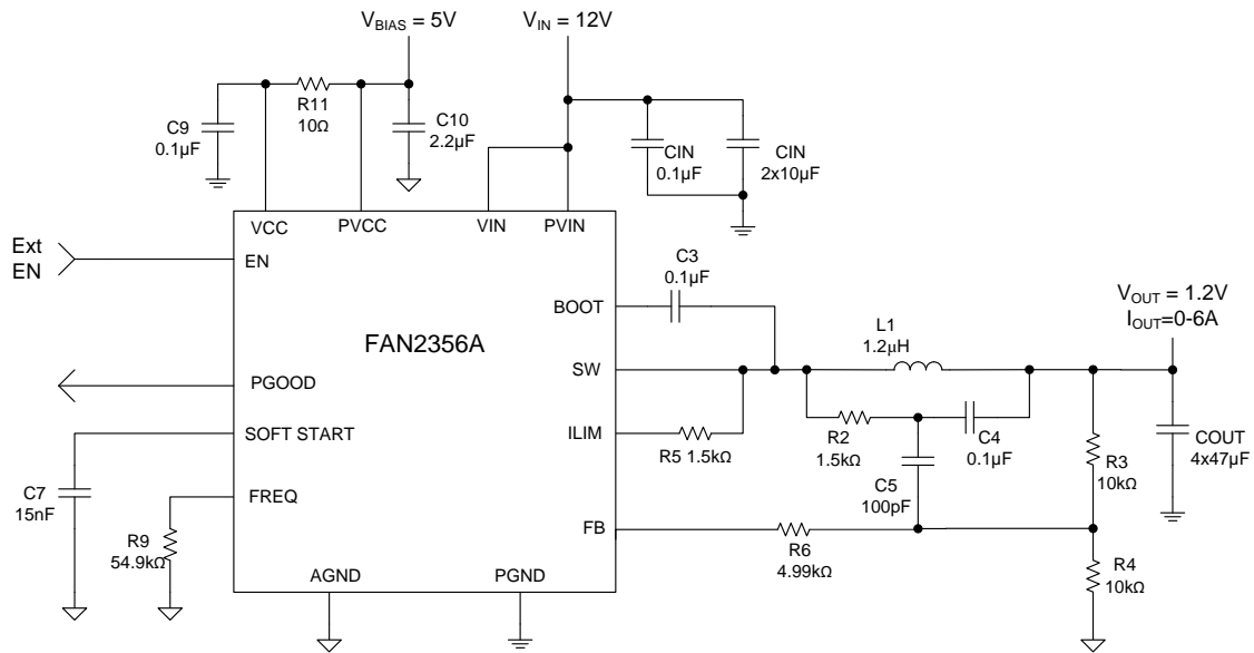
Figure 1. Typical Application
