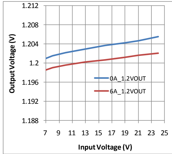
Figure 12. Line Regulation
