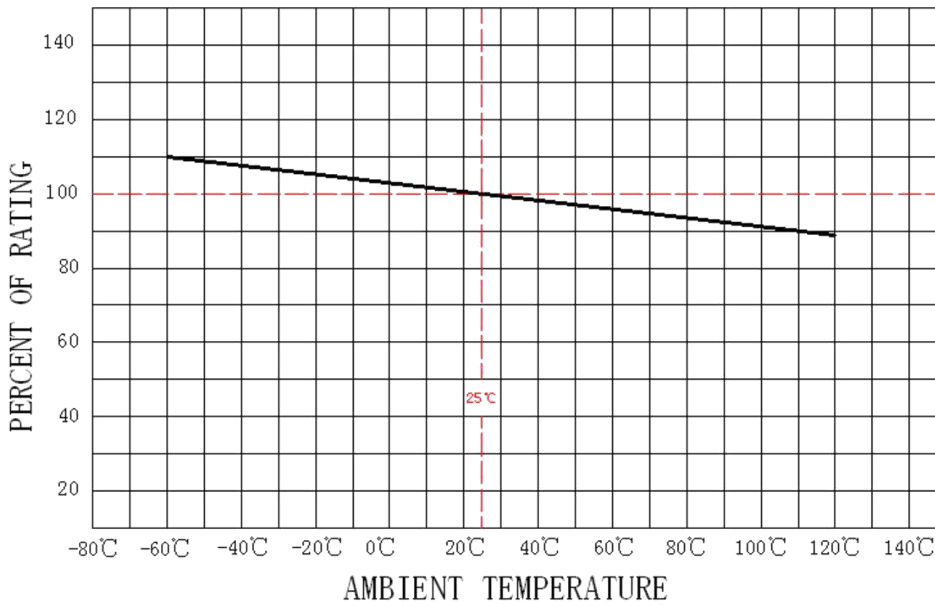
Temperature-Current curve:
