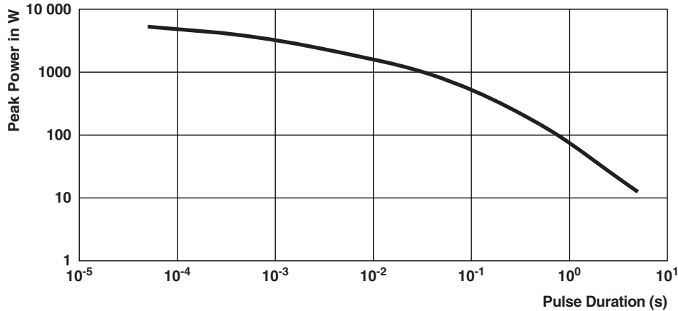
Pulse performance after a rectangular pulse of defined duration is applied
