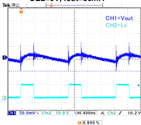
R1293KxxxA fosc=700kHz, VIN=3.0V, Vout=10V, Ta=25°C SEL=0V, Iout=80mA
