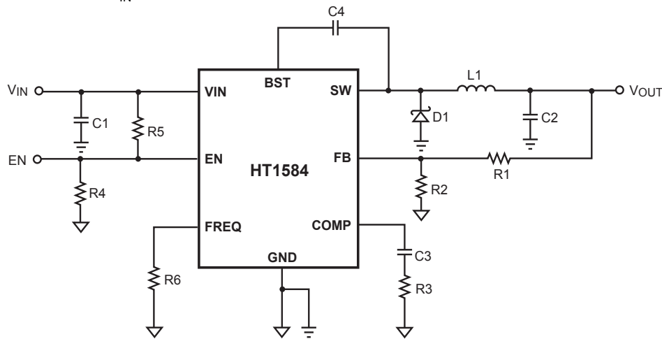
HT1584 Typical Application Circuit
