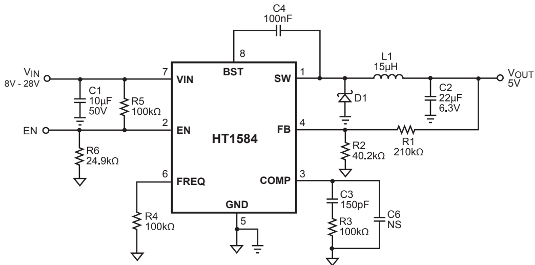
Figure 4—5V Output Typical Application Schematic
