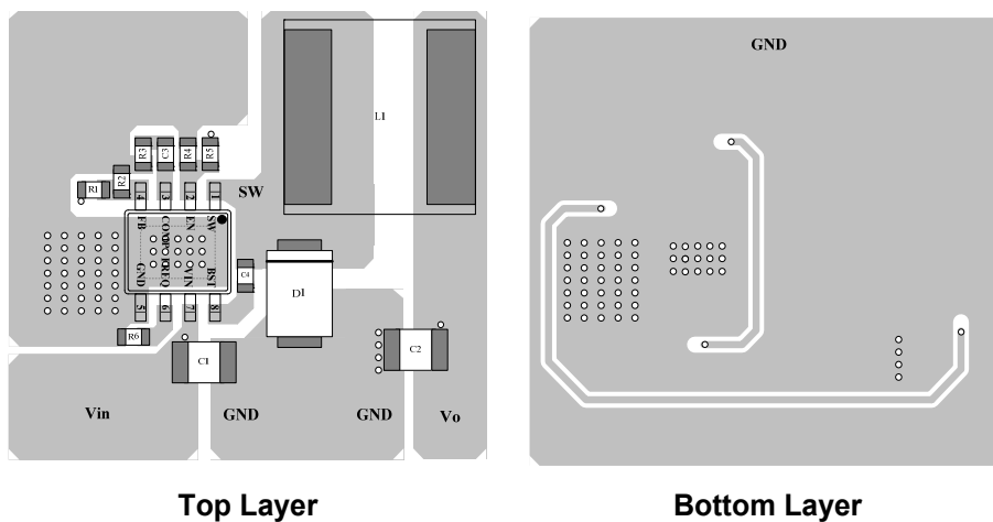
Figure 5—HT1584 Typical Application Circuit and PCB Layout Guide
