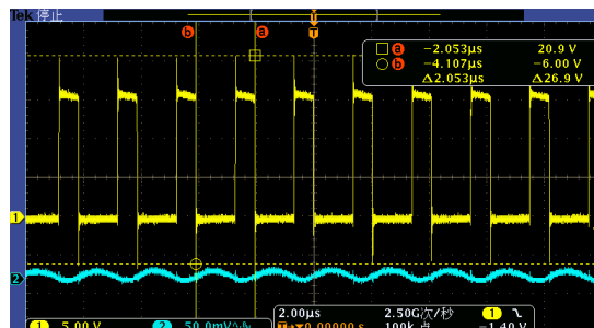
V_{PWR}=16V , I_{LOAD}=2A switching waveform
