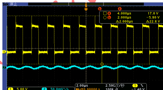
V_{PWR}=12V , I_{LOAD}=3A switching waveform
