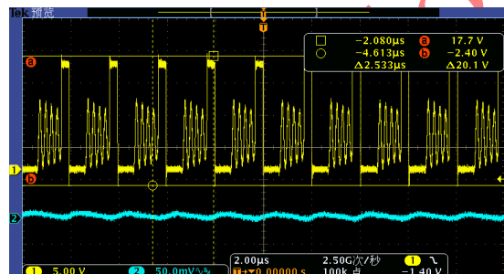
V_{PWR}=16V , I_{LOAD}=0.1A switching waveform
