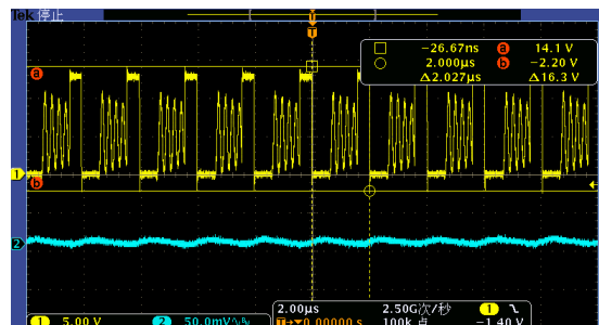
V_{PWR}=12V , I_{LOAD}=0.1A switching waveform
