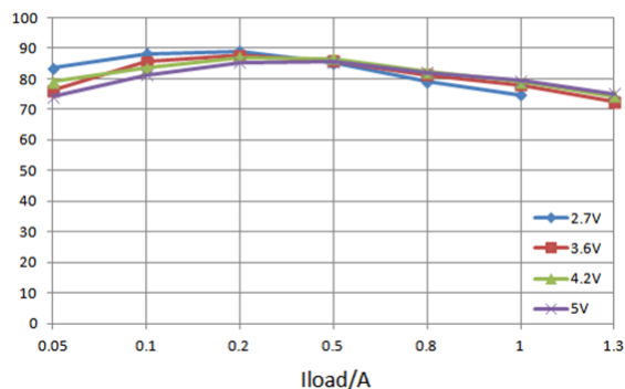
Efficiency vs Iload
