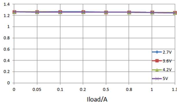
VOUT vs Iload
