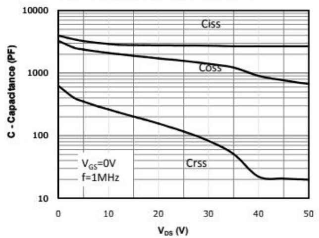
Fig 6: Capacitance Characteristics
