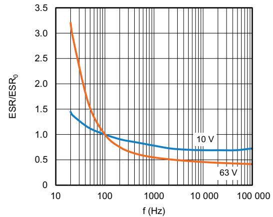
Fig. 8 - Typical multiplier of ESR as a function of frequency ( ESR_0 = typical ESR at 100 Hz at 20 °C)
