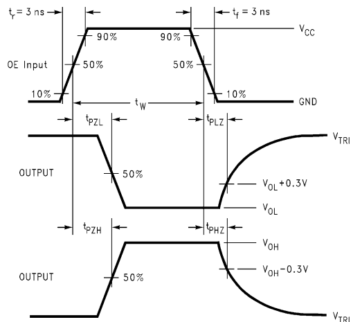
Figure 6. AC Waveforms
