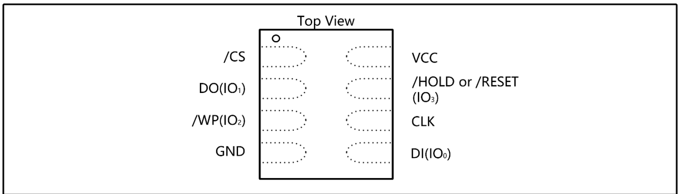
Figure 1b. MKSV064A Pad Assignments, 8-pad WSON 6x5-mm/ 8x6-mm (Package Code P/E)
