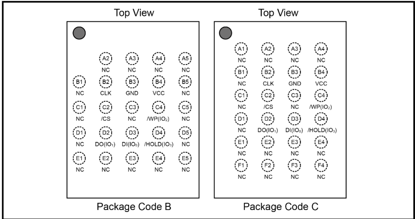
Figure 1d. MKSV064A Ball Assignments, 24-ball TFBGA 8x6-mm (Package Code B/C)
