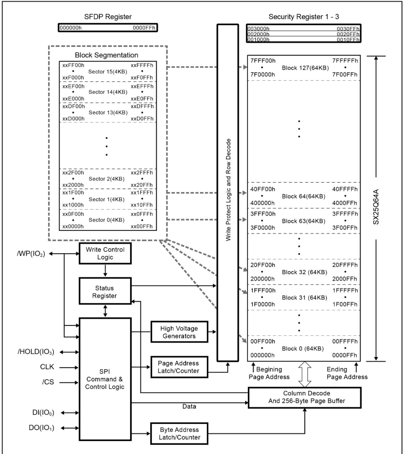
Figure 2. MKSV064A Serial Flash Memory Block Diagram
