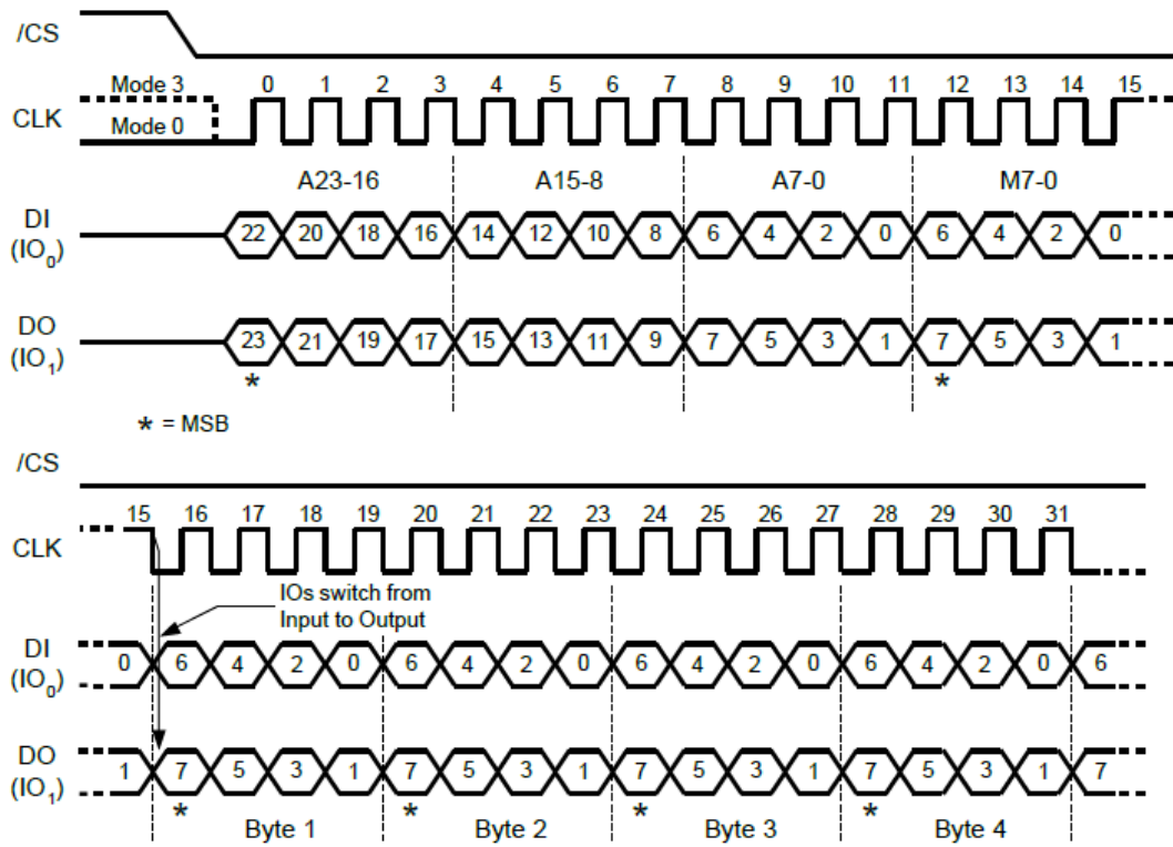
Figure 14b. Fast Read Dual I/O Instruction (Previous instruction set M5-4 = 10, SPI Mode only)
