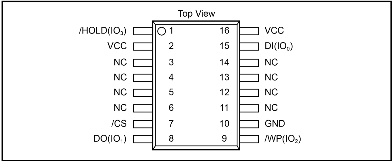
Figure 1c. MKSV064A Pin Assignments, 16-pin SOIC 300-mil (Package Code F)
