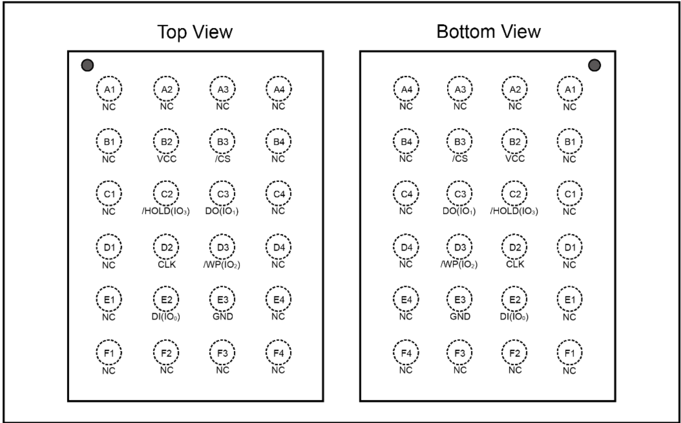
Figure 1e. MKSV064A Ball Assignments, 24-ball WLCSP (Package Code Y)
