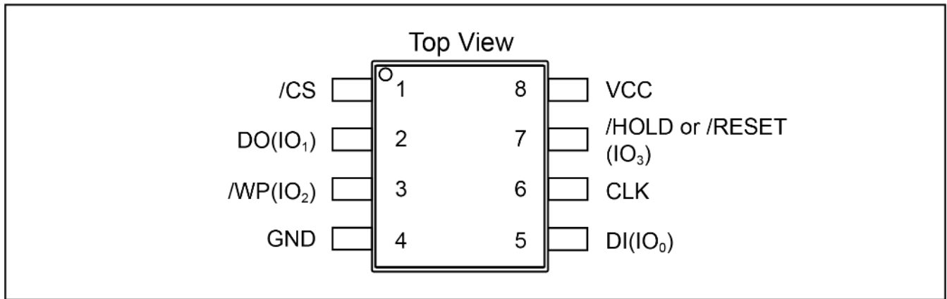
Figure 1a. MKSV064A Pin Assignments, 8-pin SOIC 208-mil (Package Code S)
