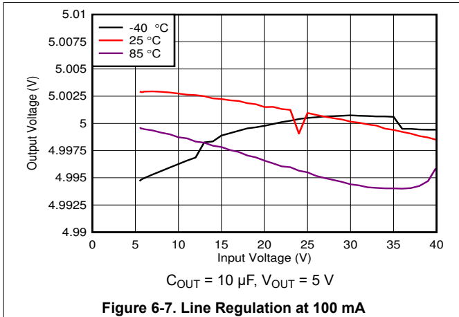
Figure 6-7. Line Regulation at 100 mA
