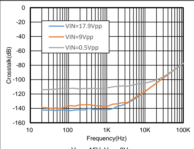
V_s = \pm 15V , V_{CM} = 0V Figure 29. Crosstalk vs. Frequency
