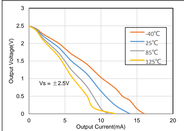
Figure 21. Positive Output Voltage vs. Output Current
