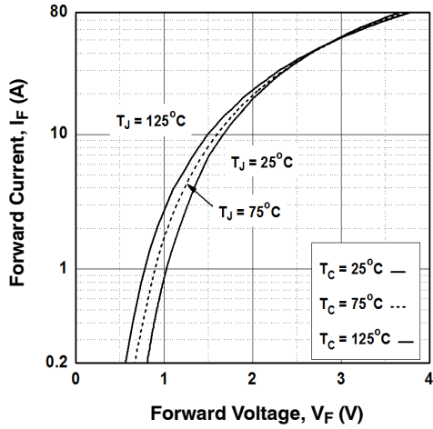
Figure 19. Forward Characteristics
