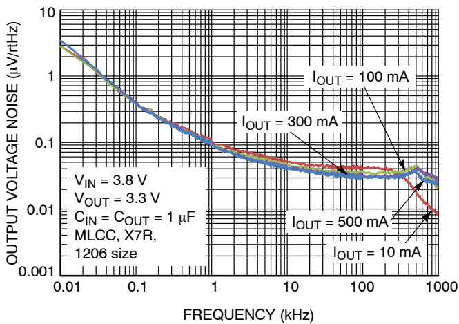
Figure 5. Output Voltage Noise Spectral Density for V_{OUT} = 3.3\text{ V} , C_{OUT} = 1\ \mu\text{F}
