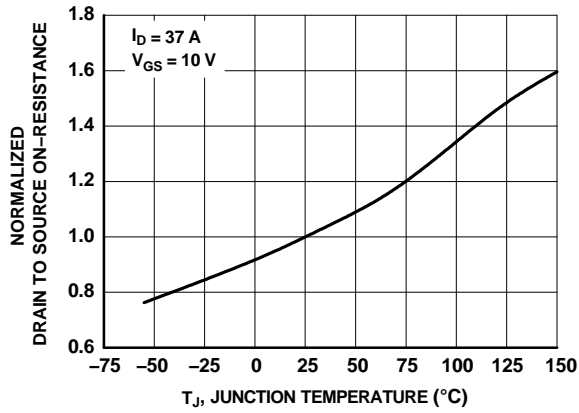
Figure 16. Normalized On-Resistance vs. Junction Temperature
