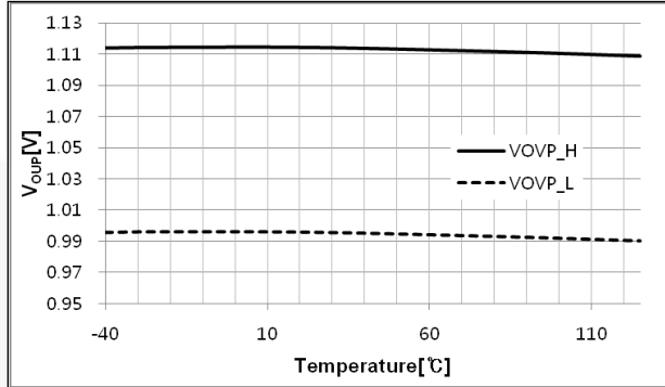
Figure 14. OVP (FB) vs. Temperature
