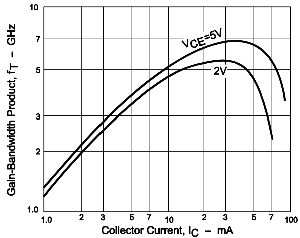
Figure 4. f_T - I_C
