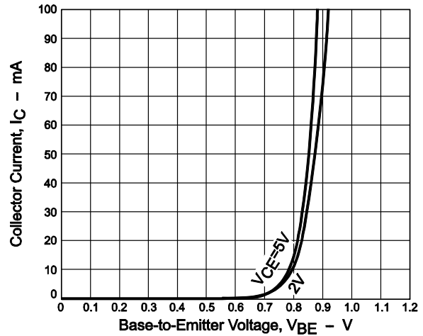
Figure 2. I_C - V_{BE}
