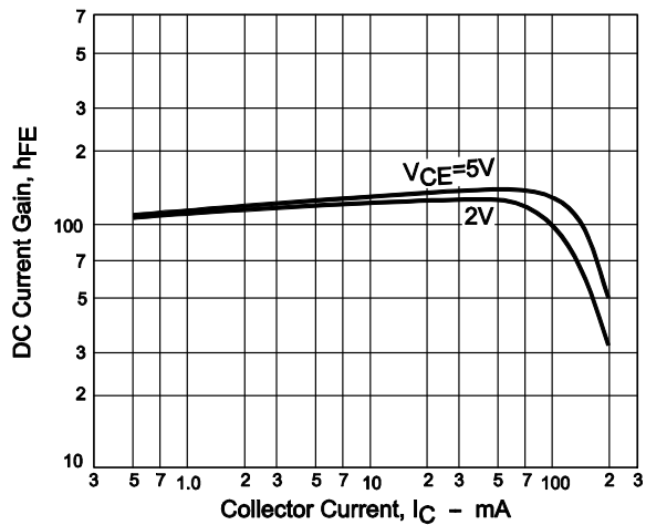
Figure 3. h_{FE} - I_C
