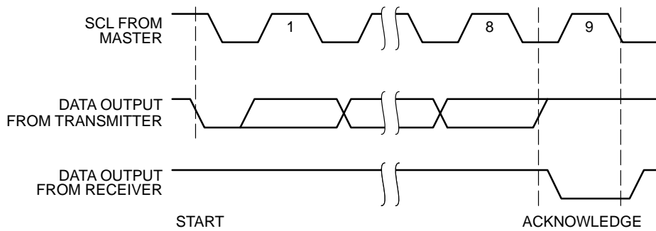
Figure 3. Acknowledge Timing
