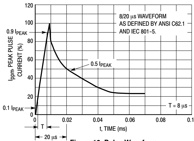
Figure 10. Pulse Waveform
