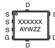
(FULL-CUT SO8FL WF) CASE 507BA DFNW5
