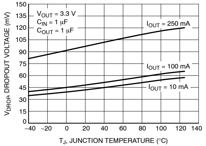
Figure 18. Dropout Voltage vs. Temperature – V_{OUT} = 3.3 V
