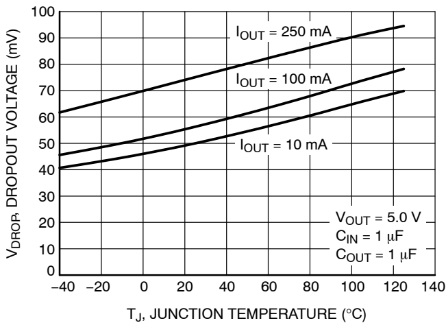
Figure 19. Dropout Voltage vs. Temperature – V_{OUT} = 5.0 V
