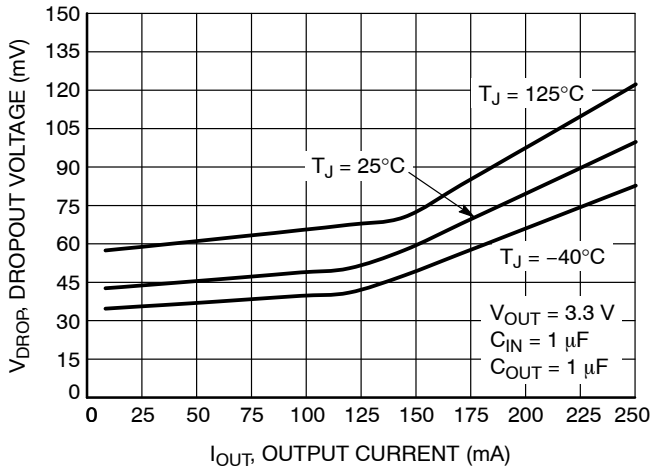
Figure 15. Dropout Voltage vs. Load Current – V_{OUT} = 3.3 V
