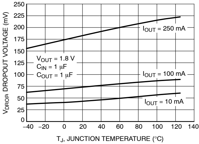
Figure 17. Dropout Voltage vs. Temperature – V_{OUT} = 1.8 V
