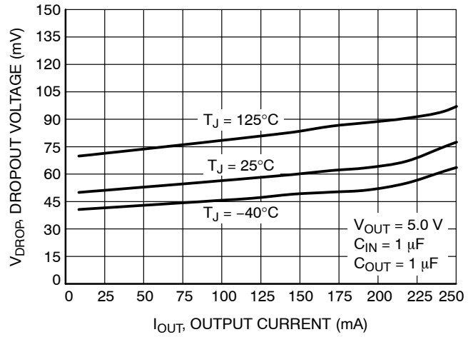
Figure 16. Dropout Voltage vs. Load Current – V_{OUT} = 5.0 V
