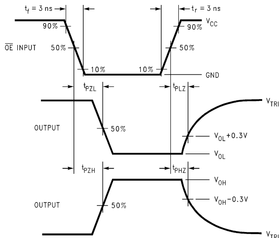
Figure 6. AC Waveforms
