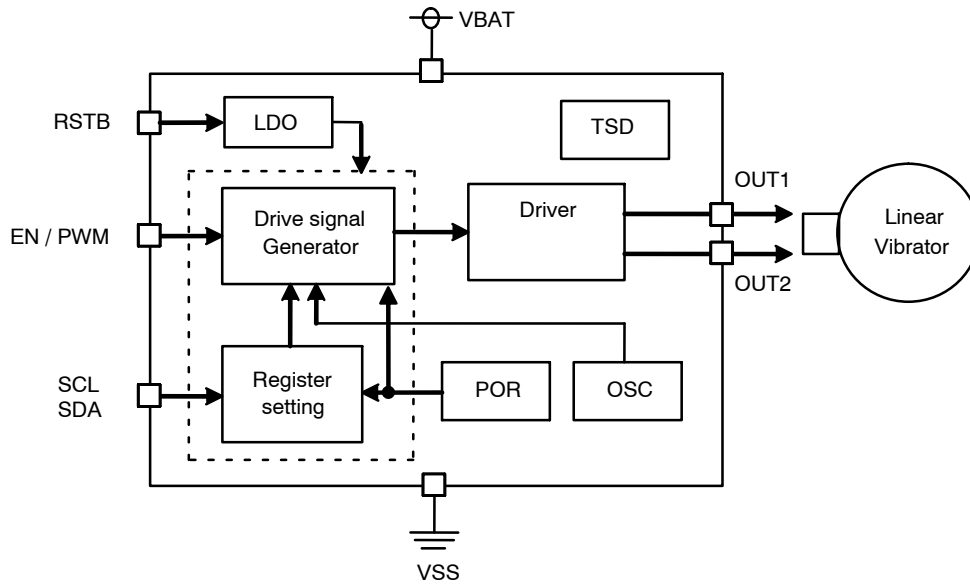
Figure 1. Block Diagram
