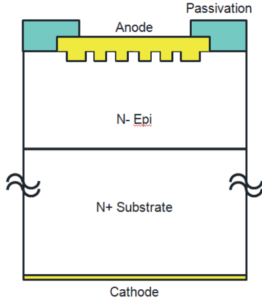
Figure 2. Cross Section
