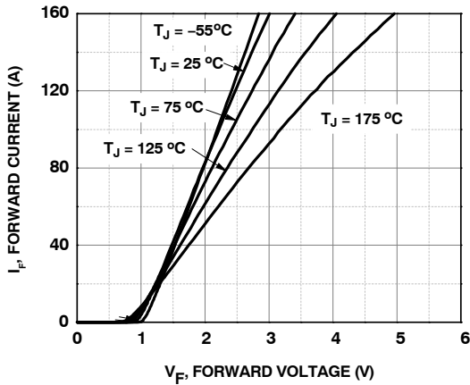
Figure 4. Forward Characteristics
