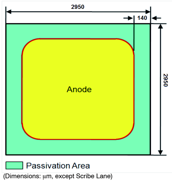
Figure 1. Die Layout
