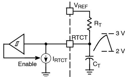
Figure 48. Oscillator Configuration
