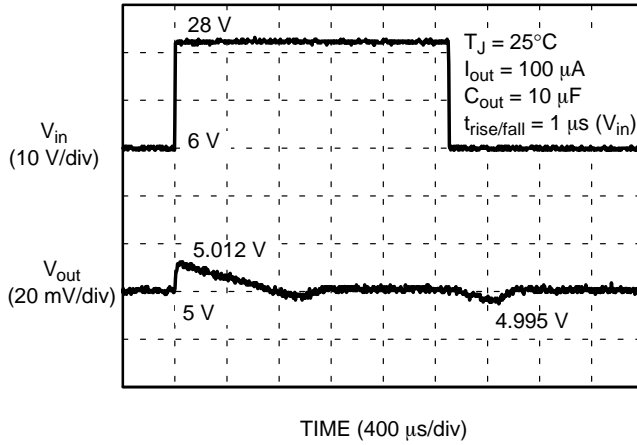
Figure 29. Line Transients
